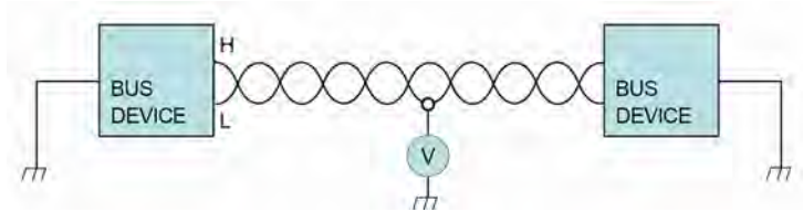
Fig. 26: Bus pin fault protection
