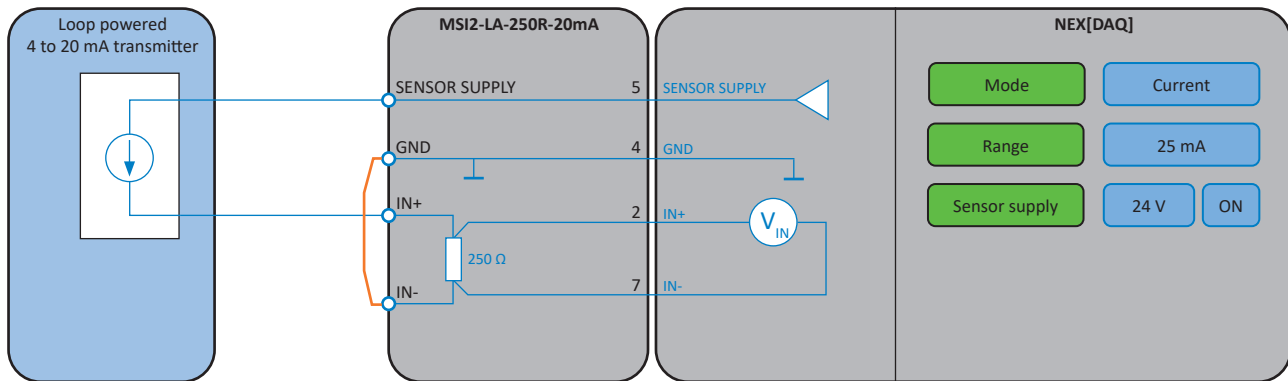
Fig. 12: Sensor connector MSI2-LA-250R-20mA
