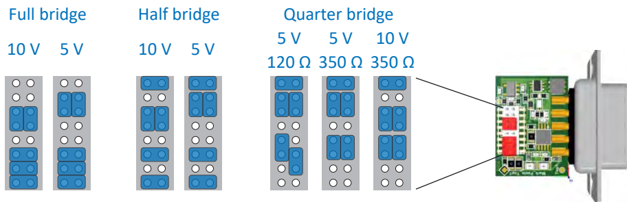
Fig. 8: Jumper settings
