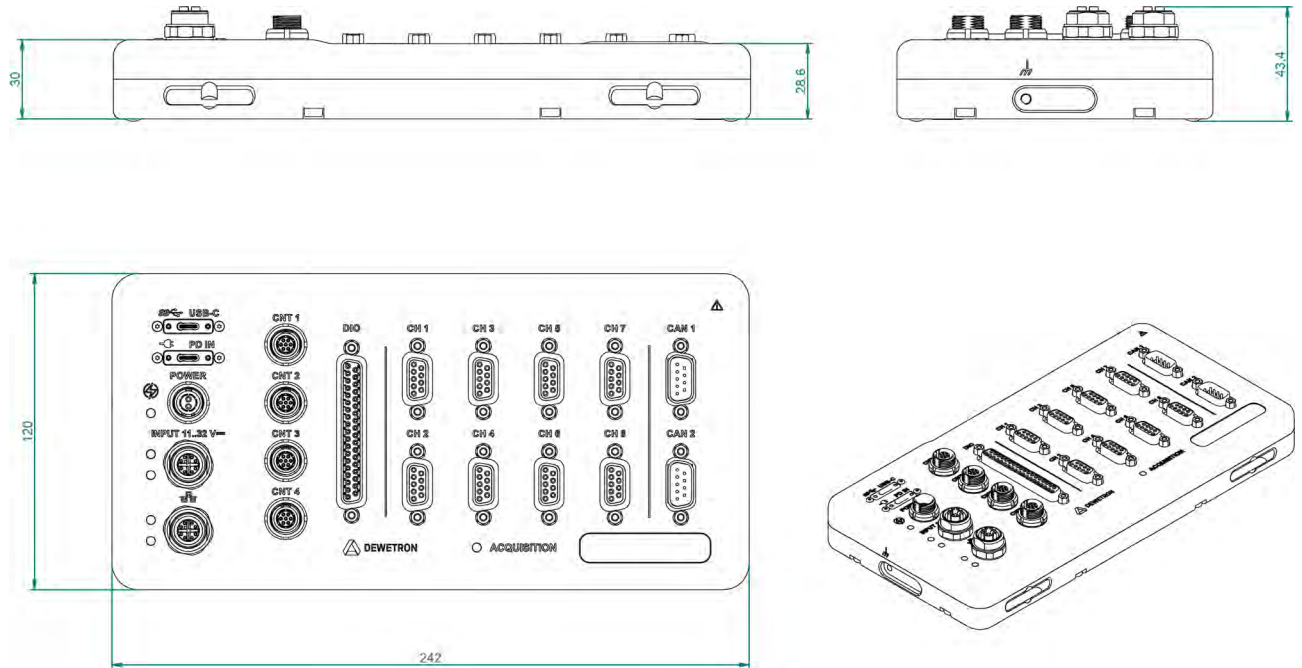
Fig. 1: Dimensions NEX[DAQ]
