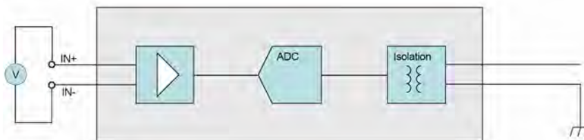
Fig. 25: Overvoltage protection
