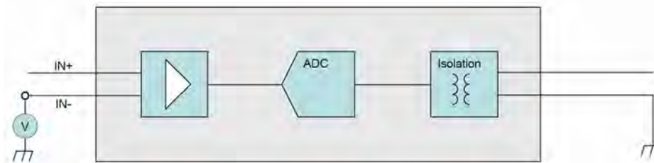
Fig. 21: Isolation voltage
