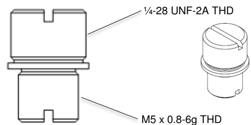
1/4-28:M5 Male Stud P/N AC-D03664
