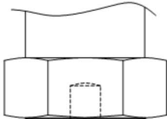
1/4-28 UNF Female THD (Integrated part of the sensor)
