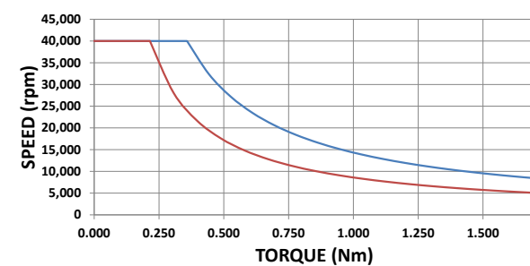
HD-515 HIGH SPEED
