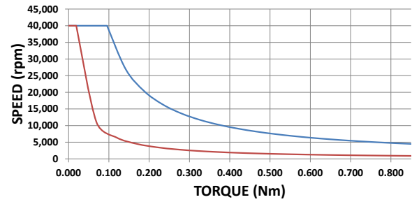
HD-510 HIGH SPEED
