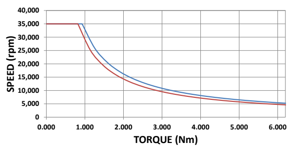
HD-715 HIGH SPEED
