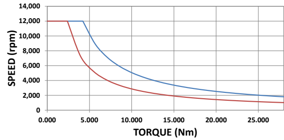
HD-810 HIGH SPEED
