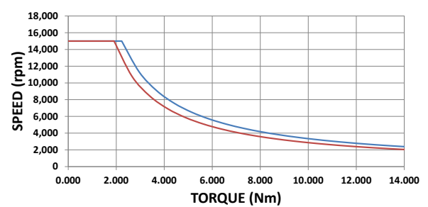
HD-815 HIGH SPEED
