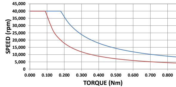
HD-505 HIGH SPEED
