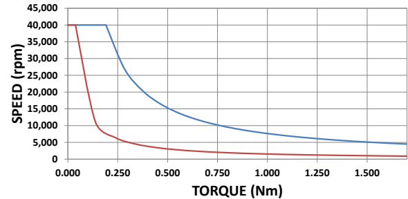
HD-515 HIGH SPEED
