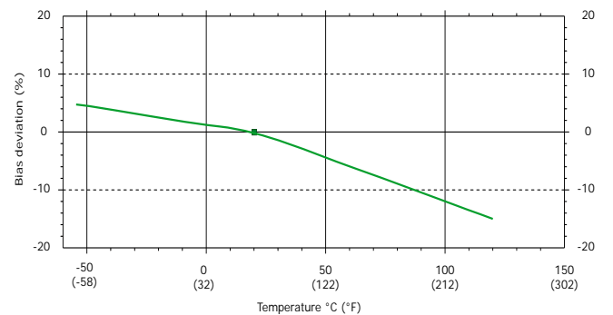
Fig 2 : DC (Bias) deviation versus temperature
