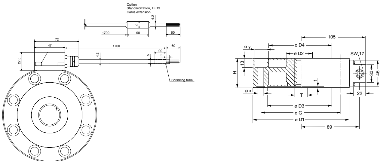
Dimensional drawing 4 – Measuring ranges from 0 ... ±100 kN up to 0 ... ±200 kN | from 0 ... ±22.5 klbs up to 0 ... ±45.0 klbs
