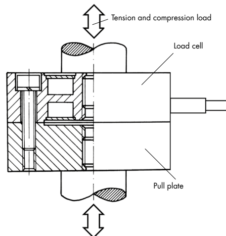
Sensor with pull plate
